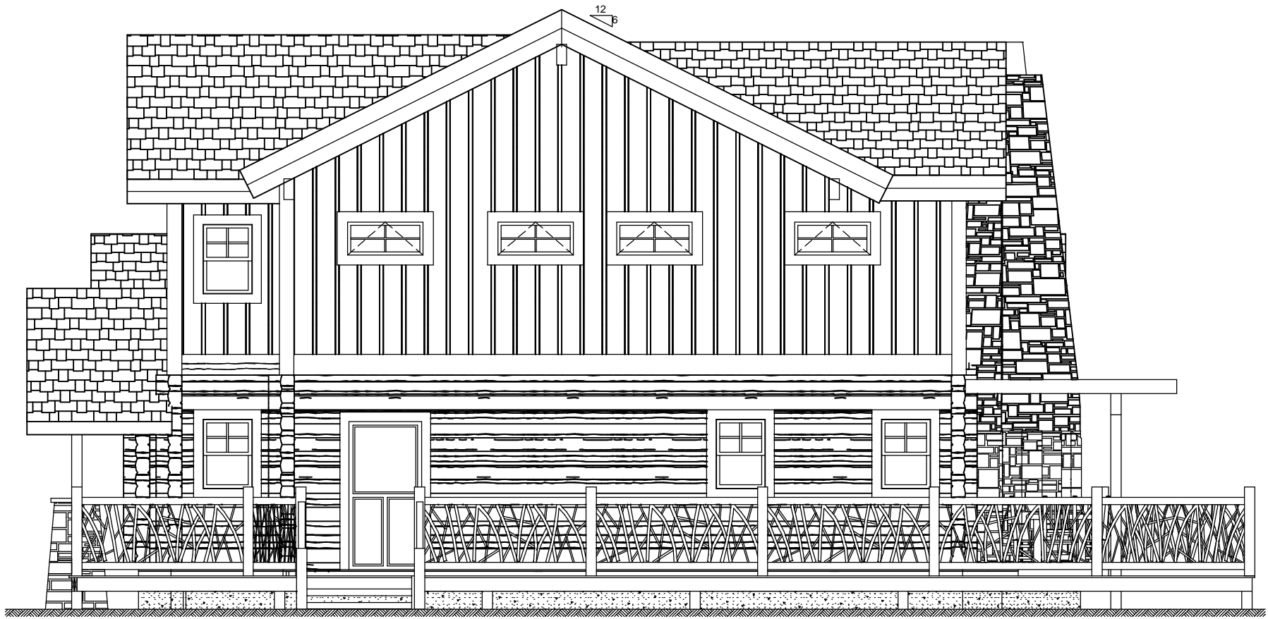
LEFT ELEVATION
