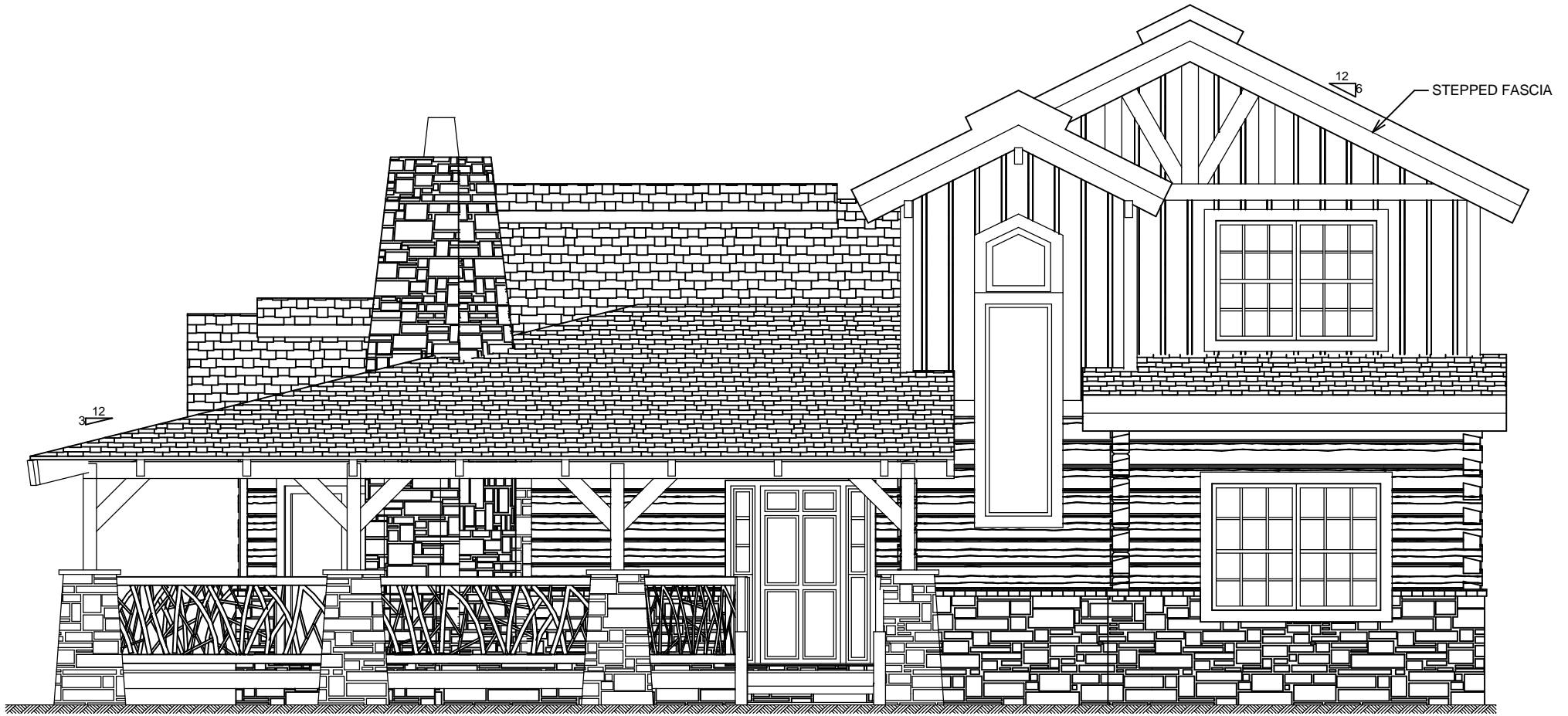
FRONT ELEVATION
