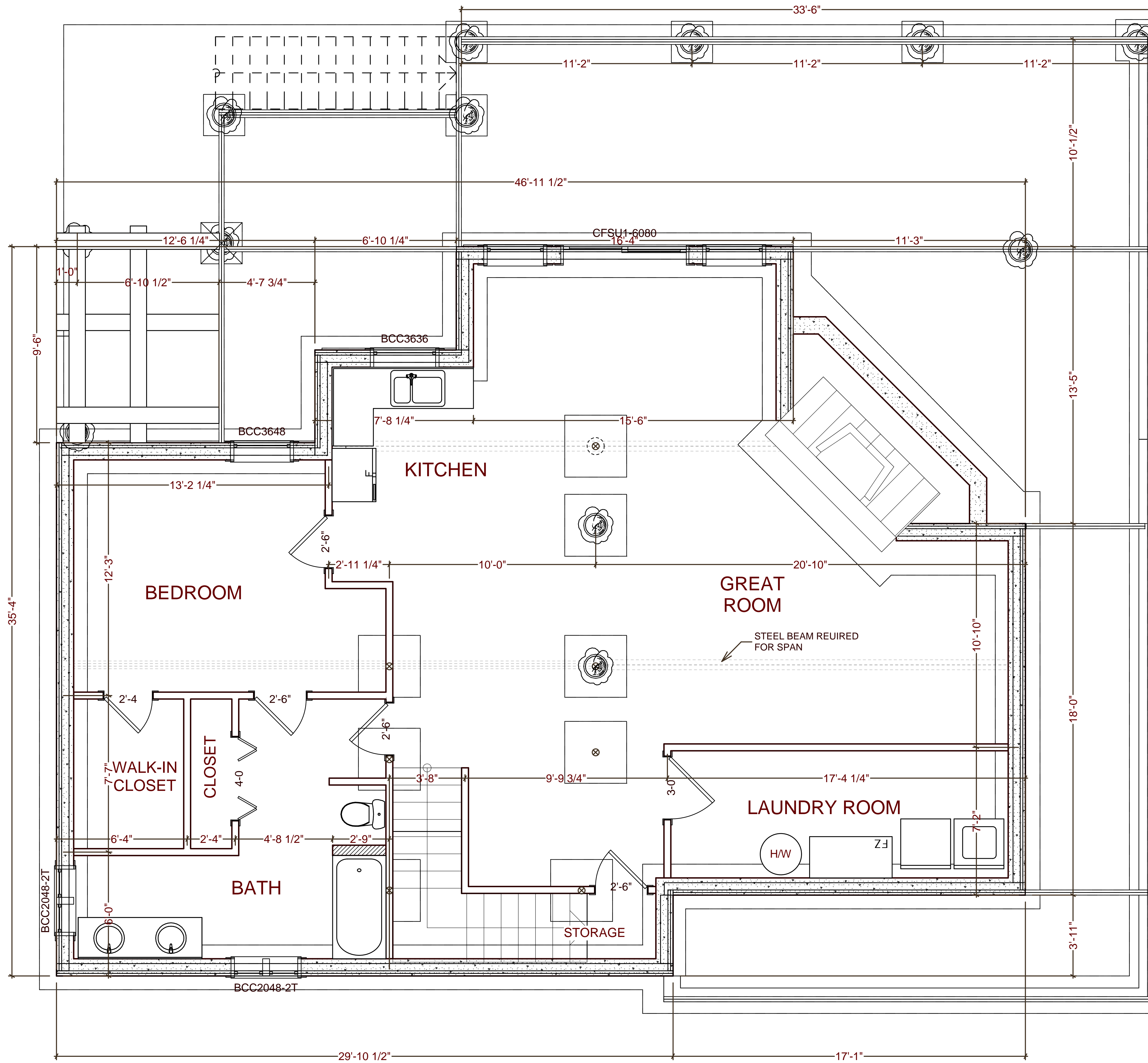
LOWER LEVEL PLAN
